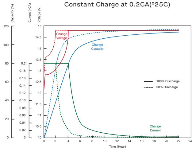
Charging Characteristics Constant Charge at 0.2CA(°25C)
