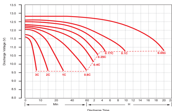
Discharging Characteristic (25°C)
