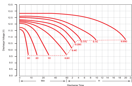
Discharging Characteristic (25°C)
